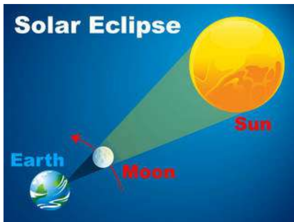
Figure 11.8 Solar Eclipse
