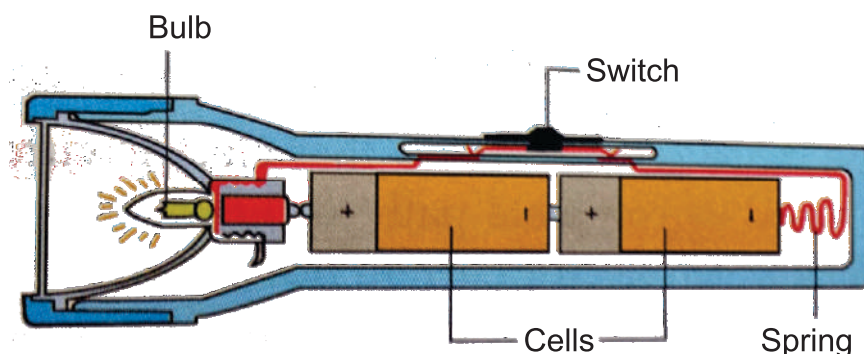
Figure 12.2 An electric Torch
