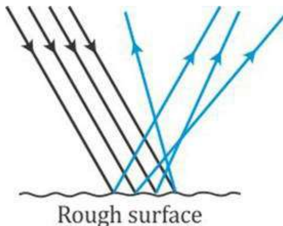
Fig. 11.16 Irregular reflection
